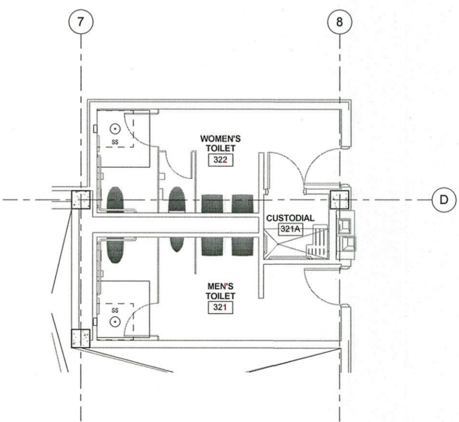
2 LEVEL 3 - Public Toilets 1/4" = 1'-0"
